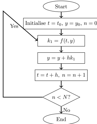
Figure 1: General flowchart for the Euler algorithm.
