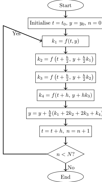
Figure 3: General flowchart for the RK4 algorithm.
