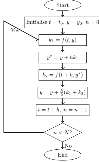
Figure 2: General flowchart for the RK2 algorithm.
